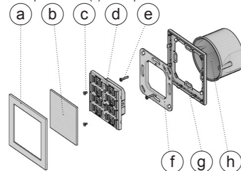
Single rectangular plate with one 60 x 60 mm window Code EK-PRS-... (to be used with rectangular version)
