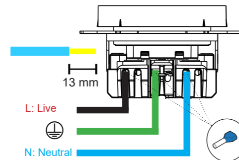
Wiring scheme for EK-PWS-FR
