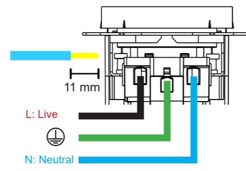
Wiring scheme for EK-PWS-FR-USB
