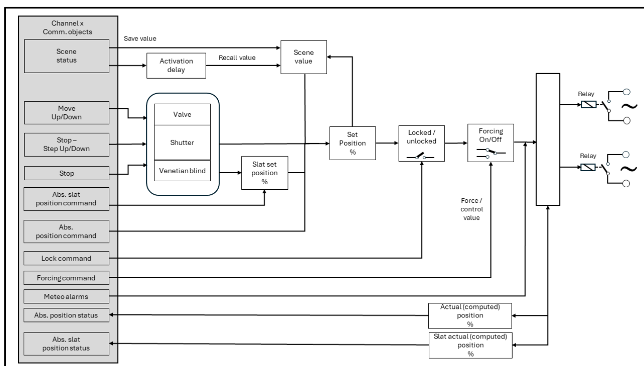
Figure 17 - Functional blocks – Coupled mode (referred to a coupled output)
