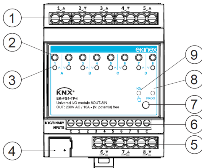
Figure 1 - Switching, display and connection elements for EK-FG1-TP-I
