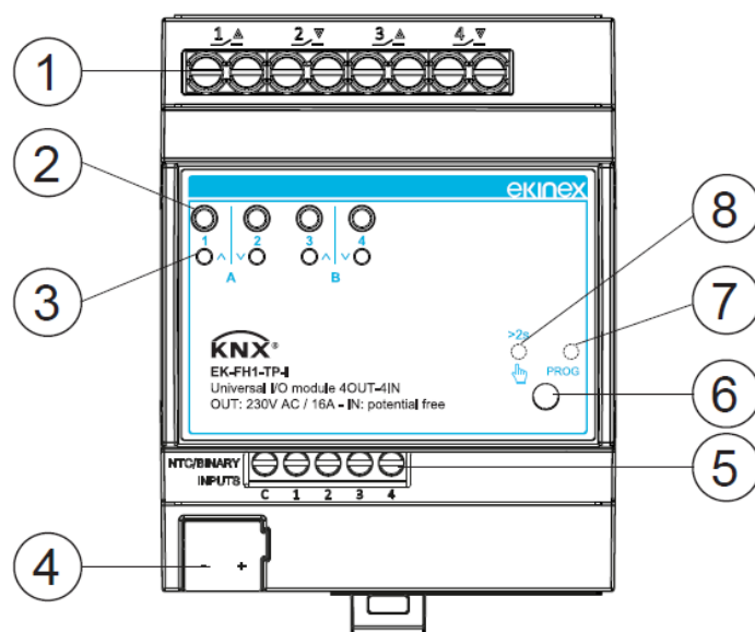
Figure 3 - Switching, display and connection elements for EK-FH1-TP-I
