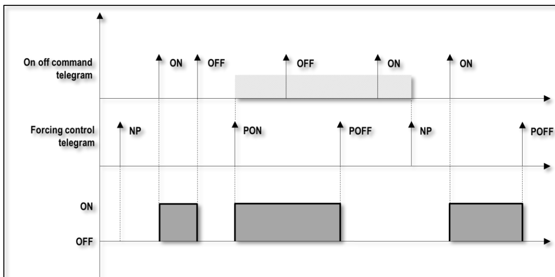
Figure 10 - Forcing function
