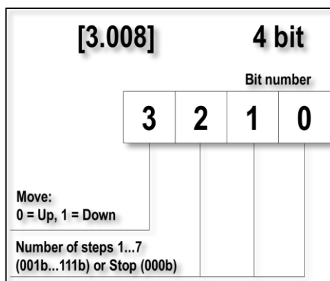
Figure 15 - Shutter control with dimming
