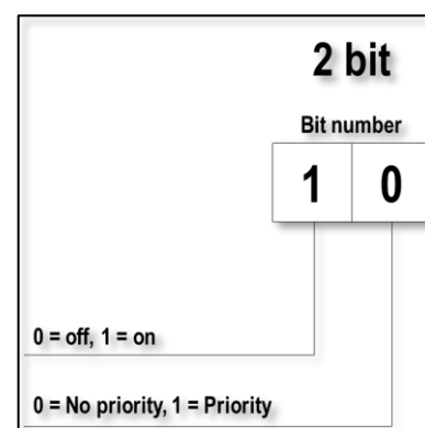
Figure 11 - Force command bits
