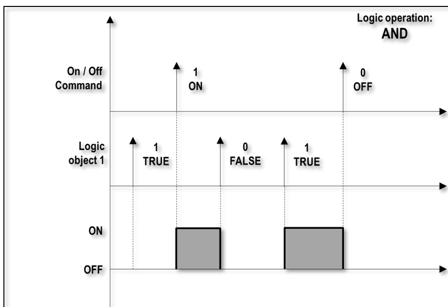
Figure 20 - Logic AND function
