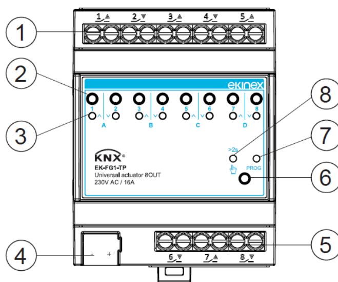
Figure 1 - Switching, display and connection elements for EK-FG1-TP
