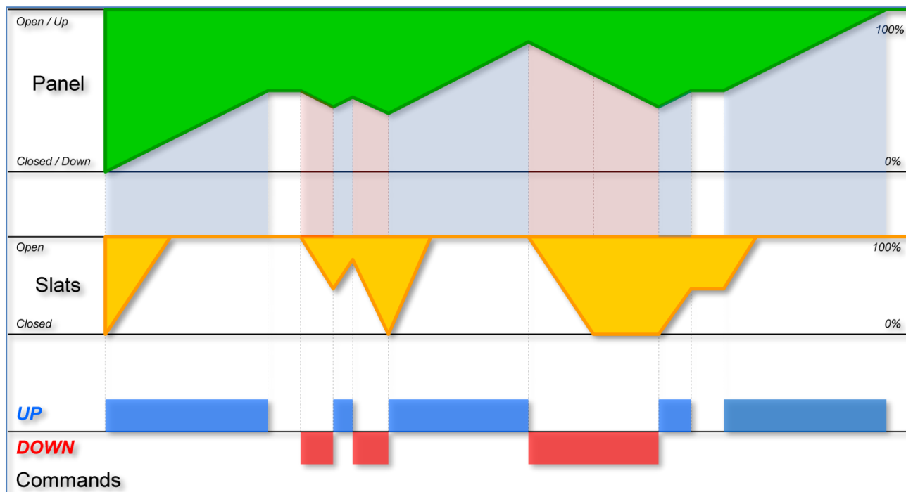
Figure 16 - Venetian blind control diagram
