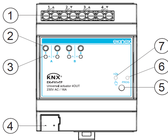
Figure 3 - Switching, display and connection elements for EK-FH1-TP
