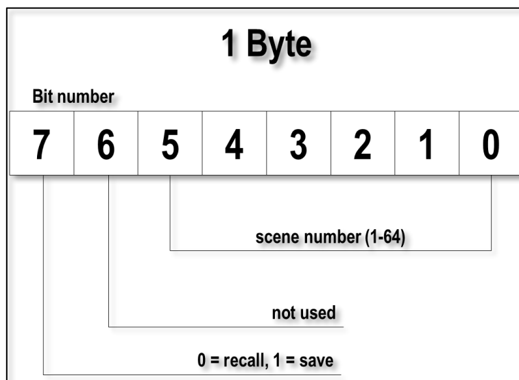
Figure 12 - Scene store / recall command code
