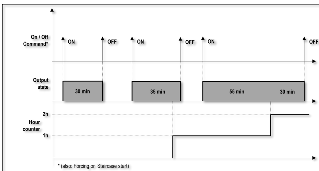
Figure 13 - Operating hours and energy counter
