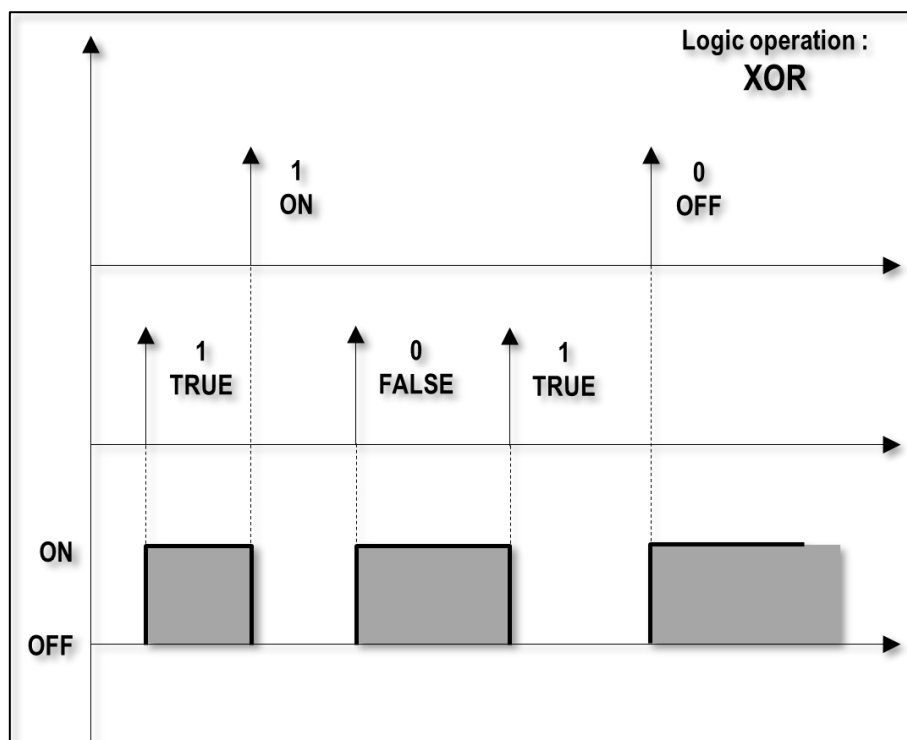
Figure 21 - Logic XOR function
