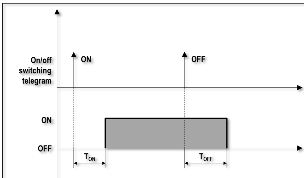
Figure 5 – ON/OFF Time delay
