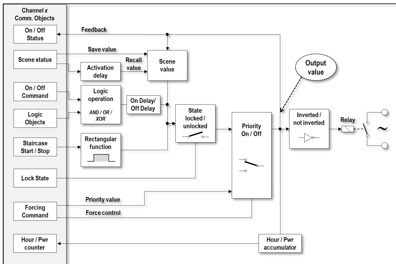
Figure 4 - Functional blocks – Independent mode (referred to a single output)
