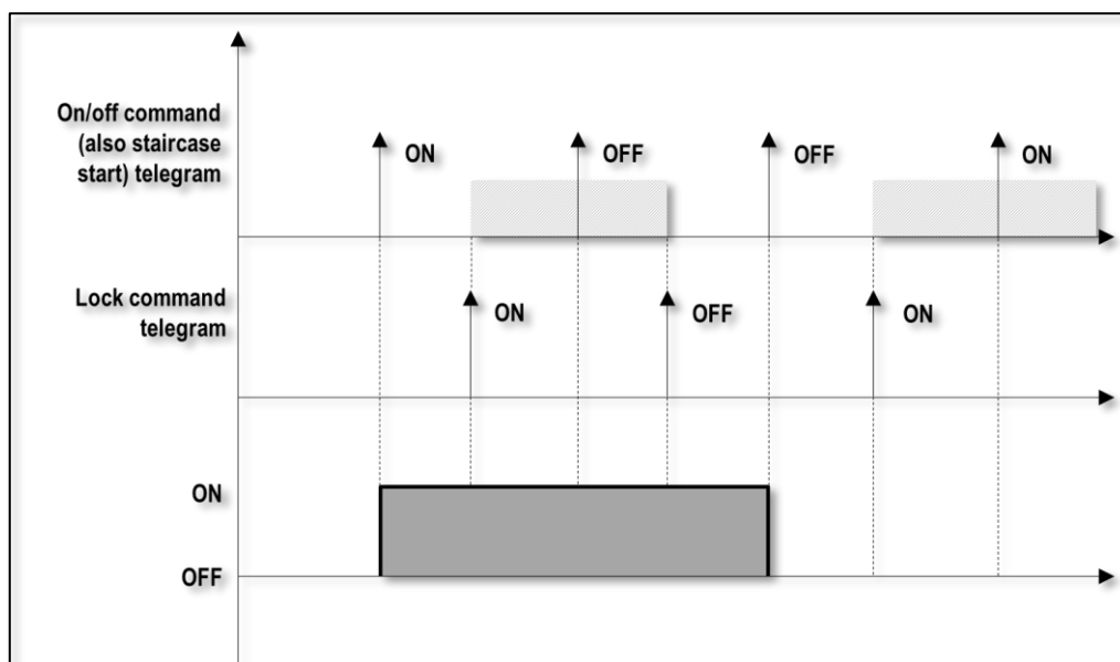
Figure 9- Lock function
