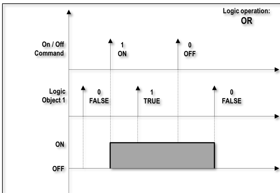
Figure 19 - Logic OR function
