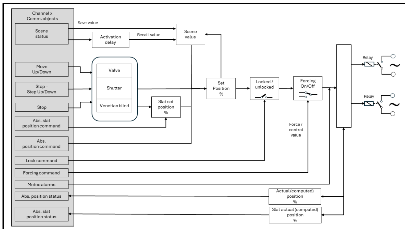
Figure 14 - Functional blocks – Coupled mode (referred to a single output)
