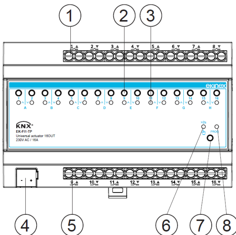
Figure 2 - Switching, display and connection elements for EK-FI1-TP
